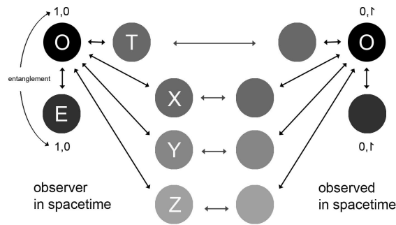
Figure 4. : 12 elementary particles and 4 interactions representing observer in interaction with observed
