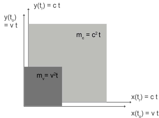
Figure 6. : creating 4-dim. spacetime with 2x2 dimensional space
