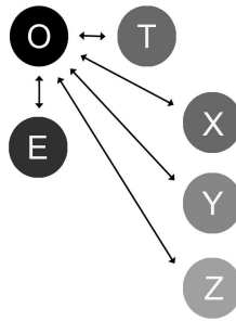
Figure 3. : Observer creating (empty) 4-dim. space-time by finding 6 elementary particles.
