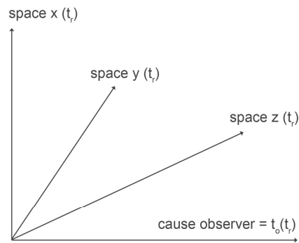
Figure 5. : creating 4-dimensional spacetime
