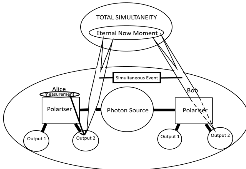
Illustration 6 : Instantaneous action through Total Simultaneity on entangled particles.
