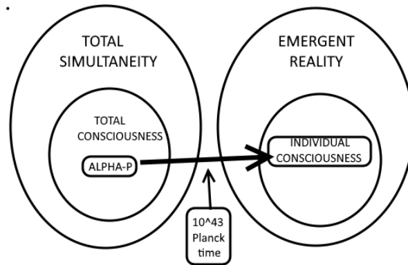
Illustration 5. The “observation” lapse between Total Simultaneity and Emergent Reality.
