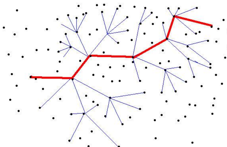
Time/Life-Line in Total Simultaneity
