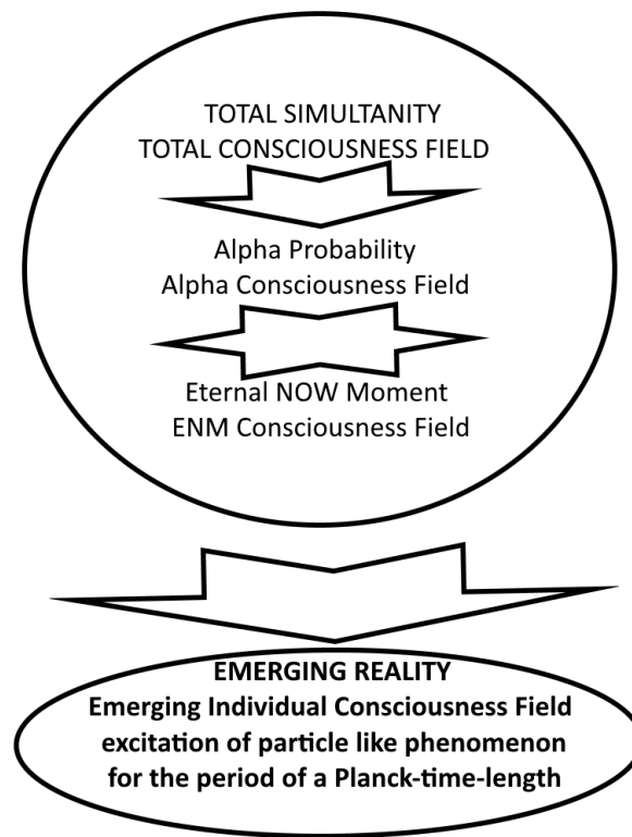
Figure 6. Consciousness as a Field
