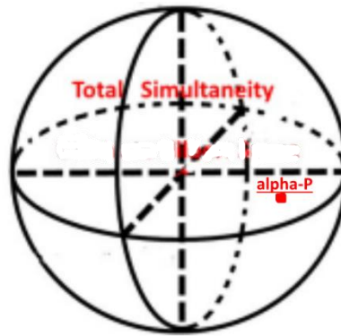
Figure 5. The specific Alpha-Probability universe as one of the infinite Probabilities in TS.
