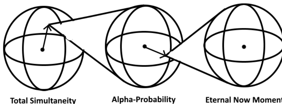
Figure 4. Both Alpha→Infinty Probabilities and Eternal Now Moments can be designed as spheres each with an infinity of vectors
