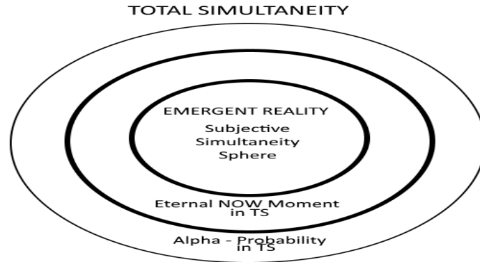
Figure 4. Subjective Simultaneity Sphere in Total Simultaneity
