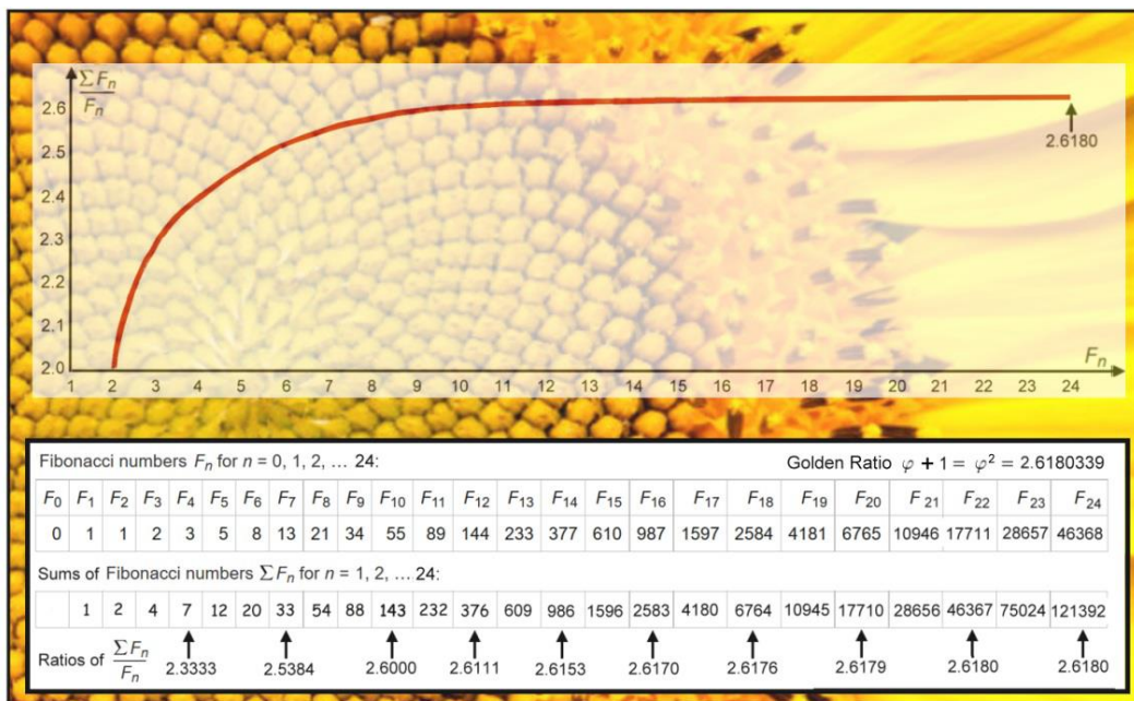
Figure 2 - Fibonacci sequence, sunflower seed patterns, and golden ratio interrelation.
