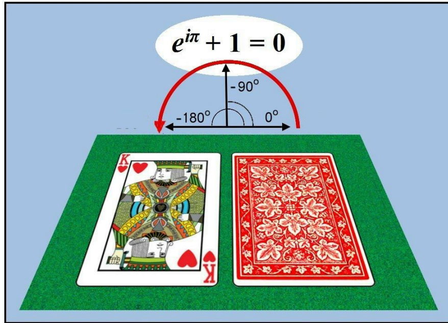
Figure 1 - Euler's identity and minus 180 degree flip of playing card.
